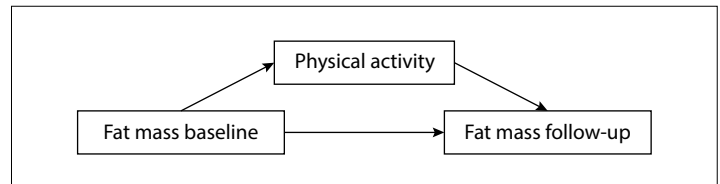
Figure 1. Theoretical model.
